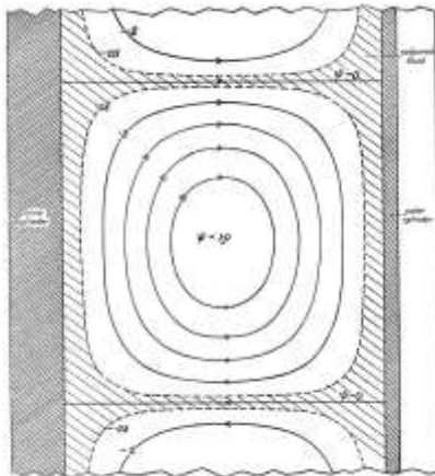
Fig. 17. Stream lines of motion after instability has set in. \Omega_1 = 10 .
