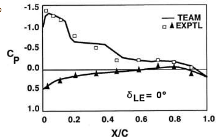
Transonic flow
