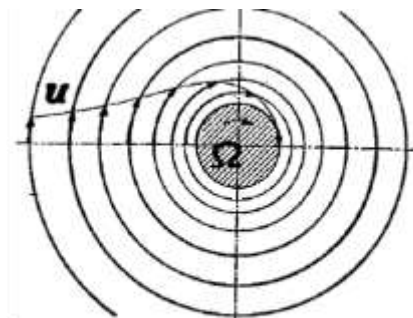
Induced velocity field of a vortex filament
