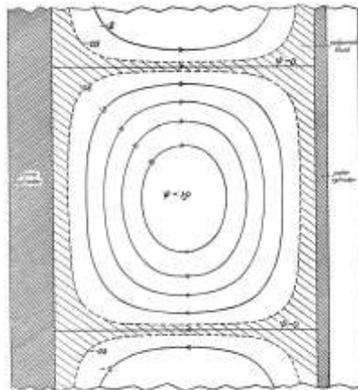
Fig. 17. Stream lines of motion after instability has set in, y position.
