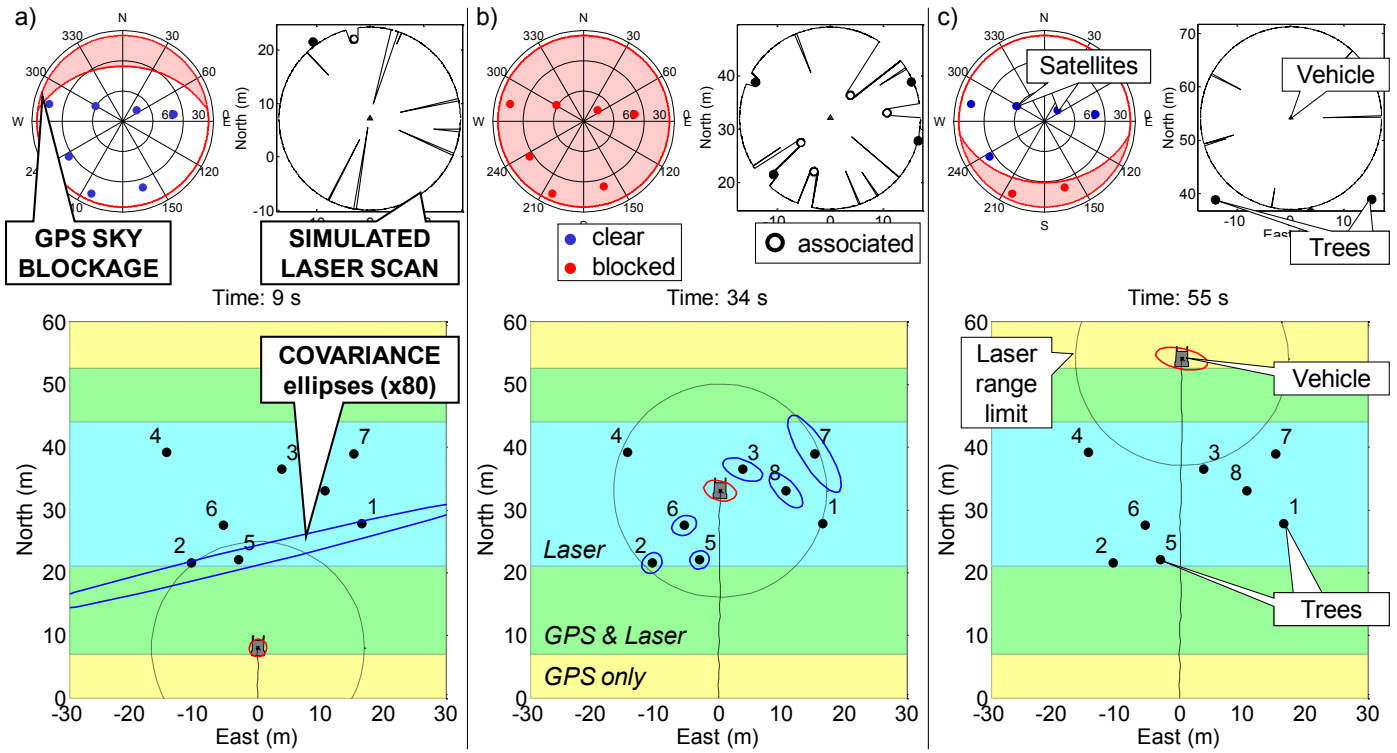
Fig. 10. Direct Simulation of the GPS/Laser Algorithm in the GPS-Denied Area Scenario: (a) the vehicle started in the GPS-available area (yellow-shaded) and enters the transitional GPS-and-laser-available area (green) where absolute landmark position is being estimated; (b) the vehicle is in the middle of the GPS obstruction and relies on laser/radar-only (blue-shaded area), so that the vehicle pose estimation error increases with travel distance; (c) the vehicle is back into a GPS available area (yellow), and the cross-track positioning drift is stopped.
