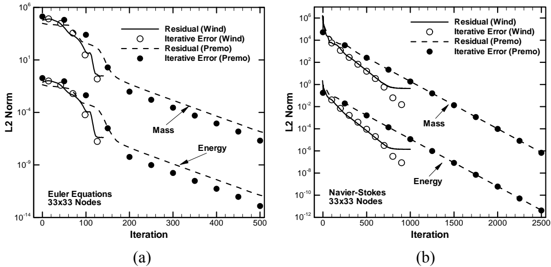
Figure 5. Global norms of the iterative convergence error and residuals for manufactured solutions of a) the Euler equations and b) the Navier-Stokes equations
