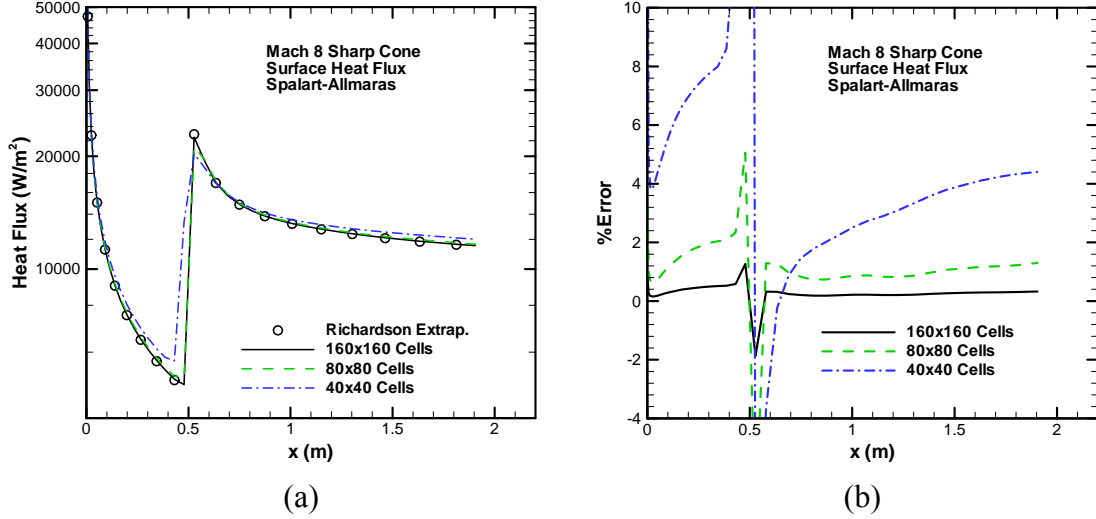
Figure 6. a) Surface heat flux and b) relative discretization error for the transitional sharp cone.
