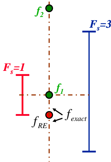
Figure 8. Factor of safety for extrapolation-based error bands
