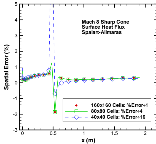
Figure 7. Normalized relative discretization error in the surface heat flux on the transitional sharp cone.
