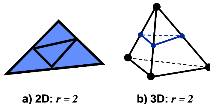
Figure 9. Refinement strategy for unstructured meshes: a) 2D triangles and b) 3D tetrahedra.
