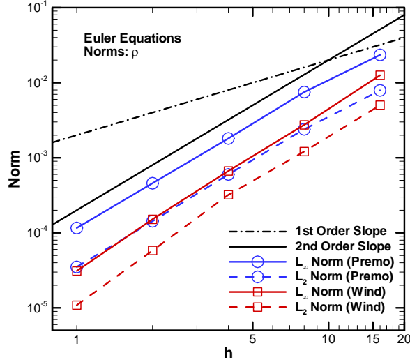
Figure 3. Global norms of the discretization error in mass density.
