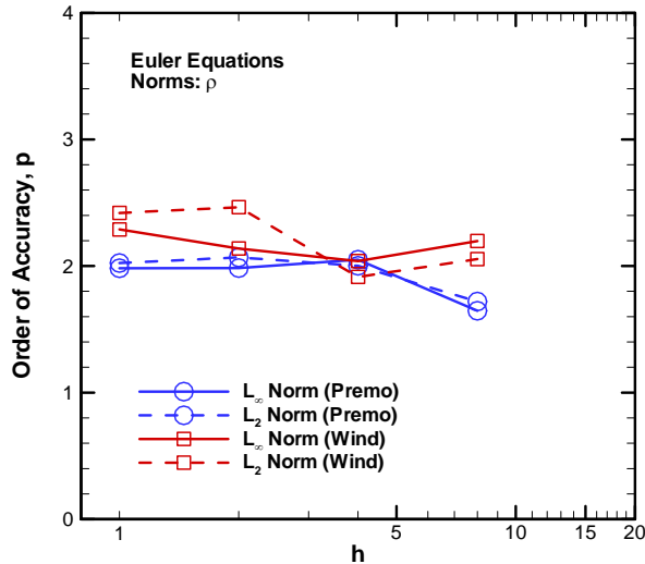
Figure 4. Observed order of accuracy for the mass density.
