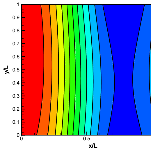
Figure 2. Analytical source term for the mass conservation equation.
