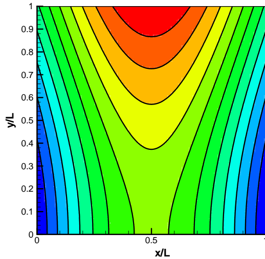
Figure 1. Manufactured solution for mass density.
