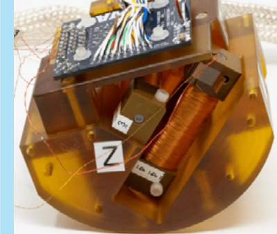
Hybrid CHIMERA sensor
